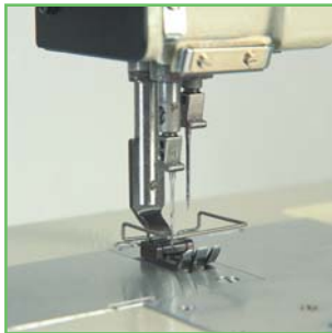
Disengageable needle bars.
